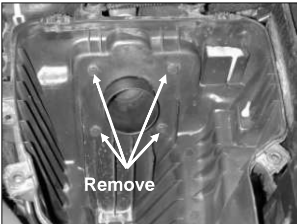
d. Remove the four screws that hold the throttle body to the lower air box.
