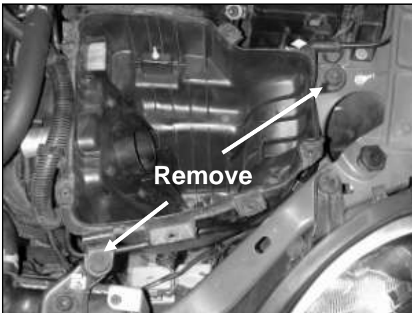
c. Remove the air filter element and the two lower air box mounting bolts.
